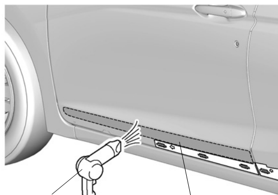
LEFT FRONT DOOR (Heat the left front door if the ambient temperature is 15°C (60°F) or below.)
