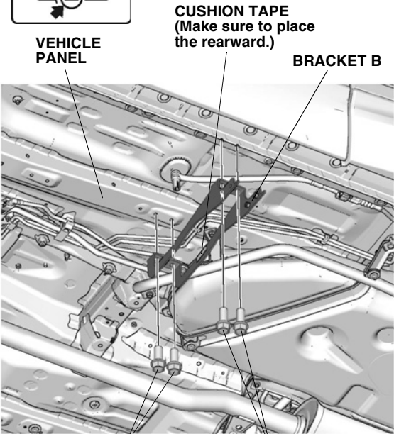
2 FLANGE BOLTS
