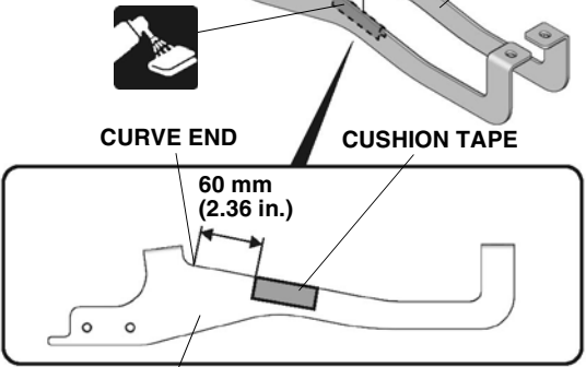
BRACKET B
