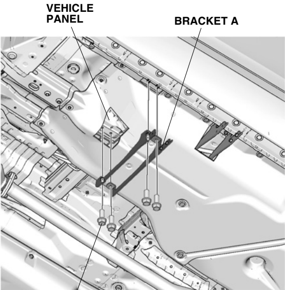
4 FLANGE BOLTS (Loosely secure.)
